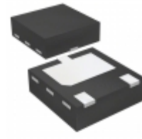
BC69-25PA,115 Nexperia USA Inc. TRANSISTOR PNP 20V 2A SOT1061
