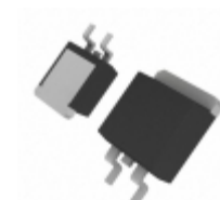
APT24M80S Microsemi Corporation MOSFET N-CH 800V 25A D3PAK
