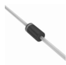
1N4764ATA SMC Diode Solutions DIODE ZENER 100V 1W DO41
