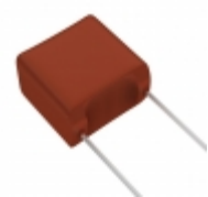
ECW-F2565HA Panasonic Electronic Components CAP FILM 5.6UF 3% 250VDC RADIAL
