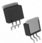
MIC2940A-3.3BU Microchip Technology IC REG LDO 3.3V 1.25A TO263-3
