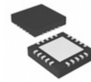
PIC16HV785-I/ML Microchip Technology IC MCU 8BIT 3.5KB FLASH 20QFN
