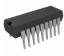
PIC16LC54C-04/P Microchip Technology IC MCU 8BIT 768B OTP 18DIP
