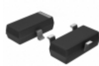
DMG301NU-7 Diodes Incorporated MOSFET N-CH 25V .26A SOT-23
