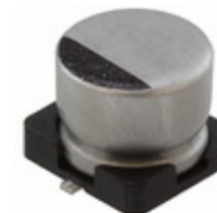
16SEV100M6.3X5.5 Rubycon CAP ALUM 100UF 20% 16V SMD
