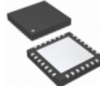
MCP23017-E/ML Microchip Technology IC I/O EXPANDER I2C 16B 28QFN
