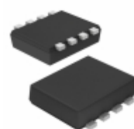
QS8J1TR Rohm Semiconductor MOSFET 2P-CH 12V 4.5A TSMT8
