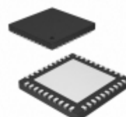
LT8601EUJ#TRPBF Linear Technology IC REG BUCK ADJ TRPL SYNC 40QFN
