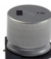
EEV-TG1K221M Panasonic Electronic Components CAP ALUM 220UF 20% 80V SMD
