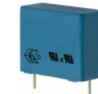
B81130C1684M EPCOS (TDK) CAP FILM 0.68UF 20% 275VAC RAD
