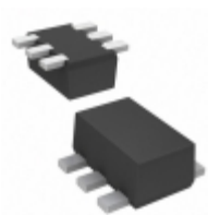
DMC964020R Panasonic TRANS PREBIAS DUAL NPN SSMINI6
