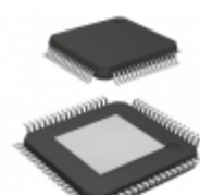
LAN9250TI/PT Microchip Technology IC ETHERCAT PHY CTRL 64TQFP
