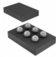
LD6938CX6/1818HF NXP USA Inc. IC REG LDO 1.8V 0.3A 6WLCSP
