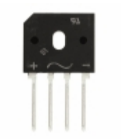
BU1210-M3/45 Vishay Semiconductor Diodes Division RECTIFIER BRIDGE 1000V 12A BU
