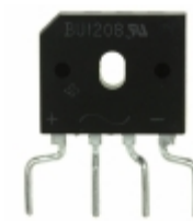
BU12085S-E3/45 Vishay Semiconductor Diodes Division RECTIFIER BRIDGE 800V 12A BU-5S
