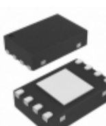
11LC040T-I/MNY Microchip Technology IC EEPROM 4KBIT 100KHZ 8TDFN
