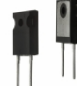
DSEP60-12A IXYS DIODE GEN PURP 1.2KV 60A TO247AD
