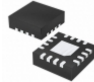
MGA-30316-TR2G Avago Technologies (Broadcom Limited) IC RF AMP 0.5W PA 3.5GHZ 16-QFN
