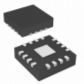
MCP23009-E/MG Microchip Technology IC I/O EXPANDER I2C 8B 16QFN
