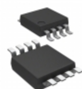
MCP73844T-840I/MS Microchip Technology IC CONTROLLER LI-ION 8.4V 8MSOP
