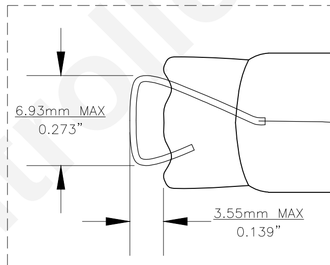
BASE DIMENSIONS
