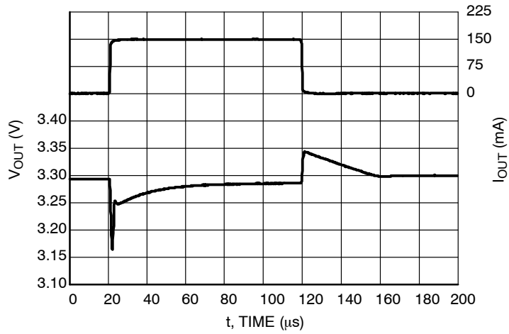
Figure 65. Load Transients, 3.3 V Version, I_{OUT} = 1 - 150 \text{ mA} , t_R = t_F = 0.5 \mu s , V_{IN} = 4.3 \text{ V} , AE = 0 \text{ V}
