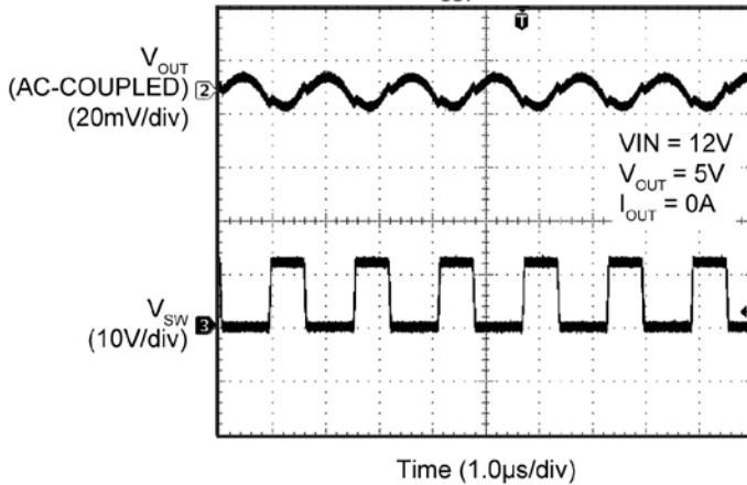
MIC28304-2 Switching Waveforms ( I_{OUT} = 0A )
