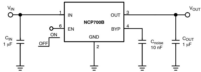
Figure 1. NCP700B Typical Application (WDFN6)
