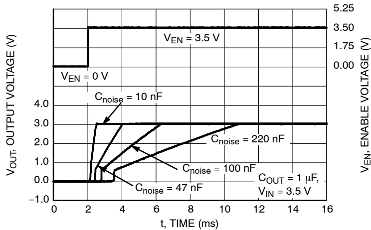
Figure 35. Turn-On Response V_{OUT} = 3 \text{ V} , C_{OUT} = 1 \mu\text{F} , I_{OUT} = 30 \text{ mA}
