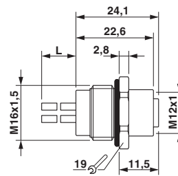
Dimensional drawing
