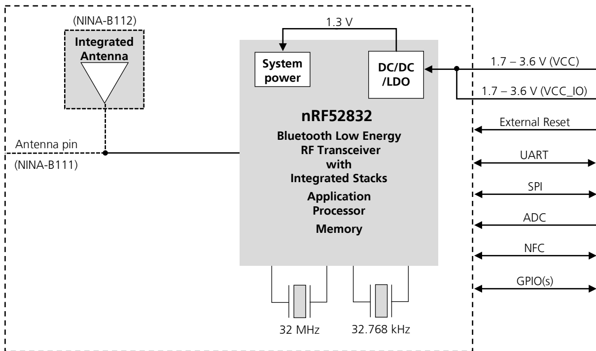
Figure 1: Block diagram of NINA-B1
