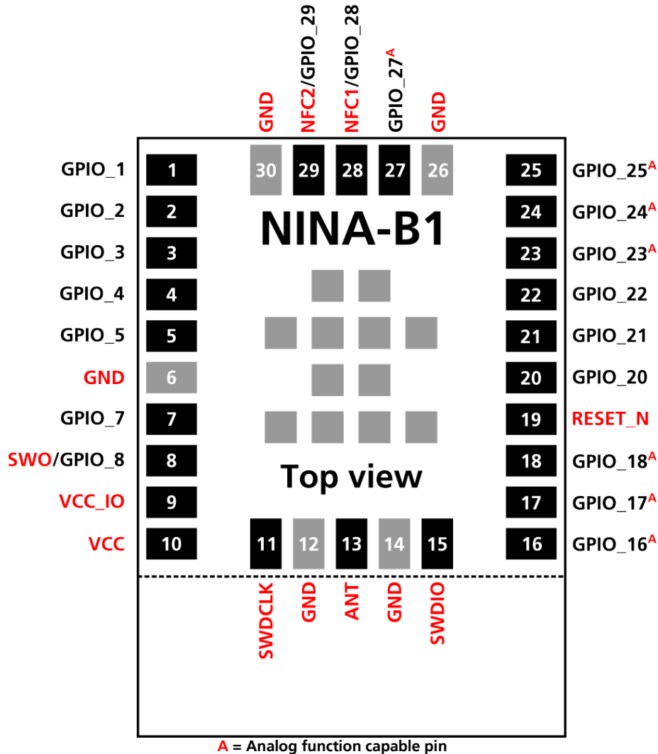
Figure 3: NINA-B1 series pin assignment (top view)
