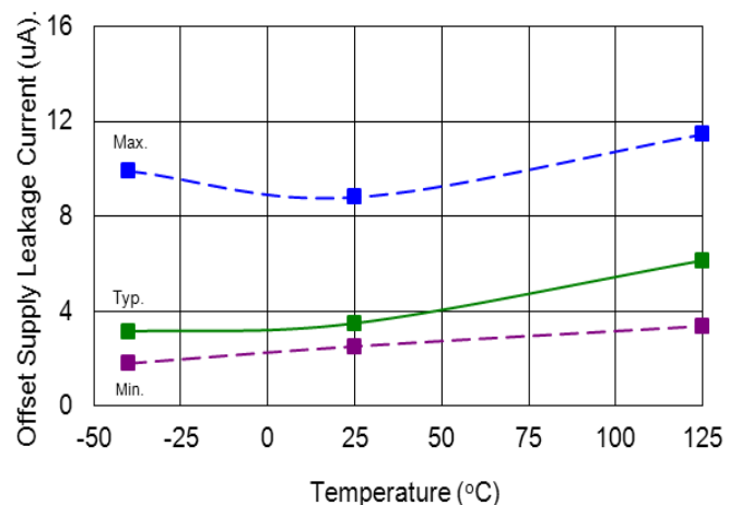
Figure 23. Offset Leakage Current vs. Temperature
