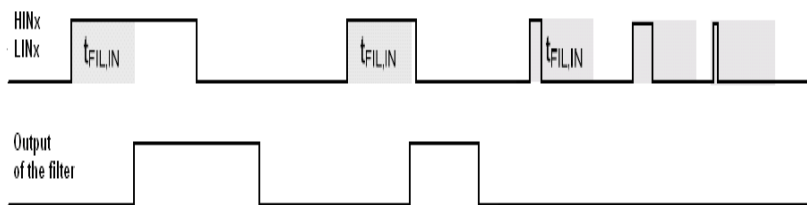
Figure 2: Input Filter
