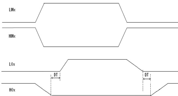
Figure 4: Dead-time Principle
