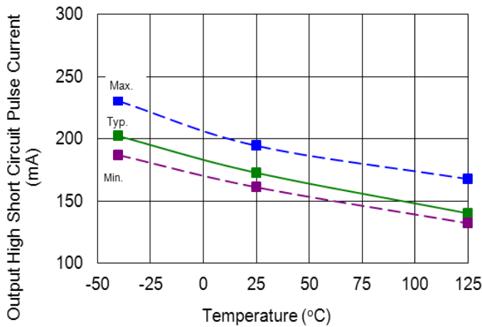
Figure 26. Output High Pulse Current vs. Temperature
