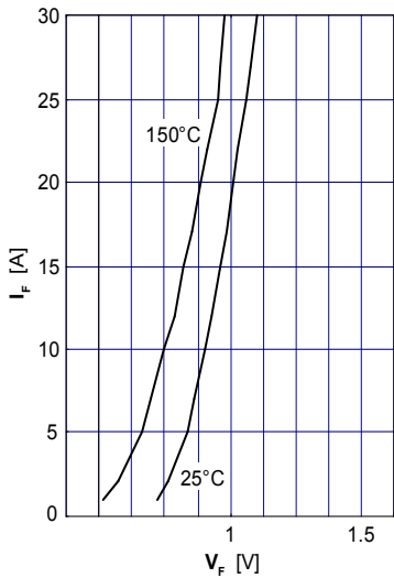
Fig. 1 Forward current versus voltage drop per diode
