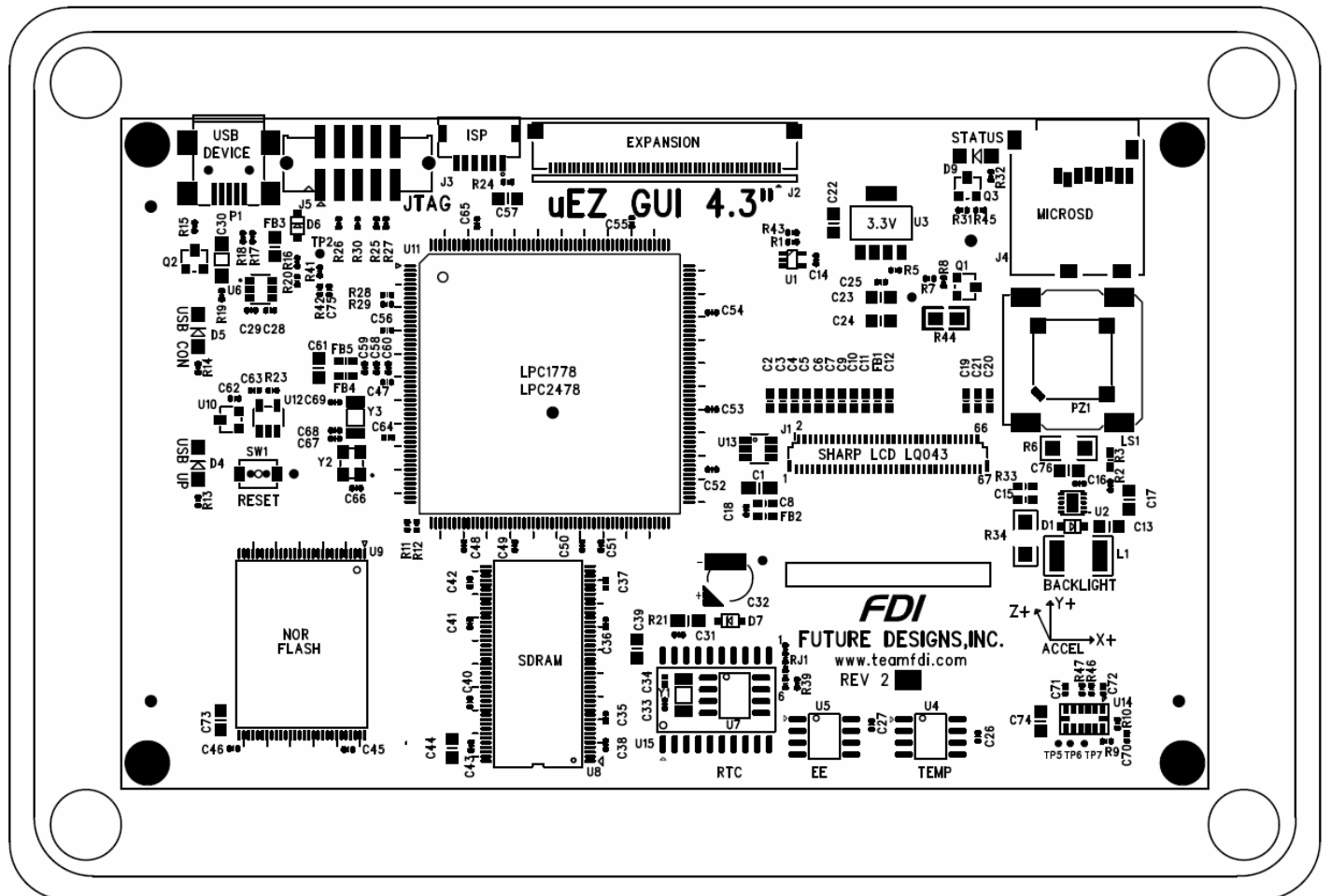
Figure 2 – uEZGUI-2478-43WQS Component View
