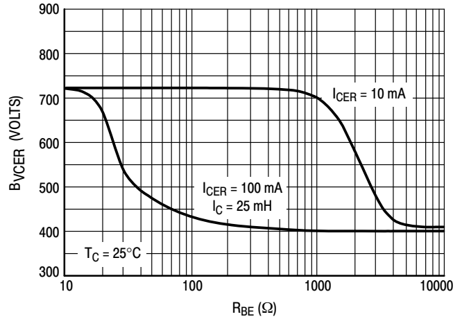
Figure 12. V CER = f(R BE )
