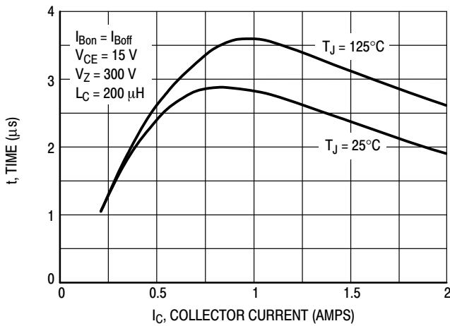
Figure 15. Inductive Storage Time, t s @ h FE = 5
