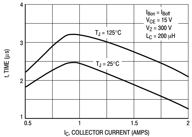
Figure 16. Inductive Storage Time, t s @ h FE = 10
